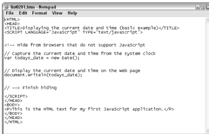
Figure 2-1: The date-and-time-stamp script as it appears in the Notepad editing window.
