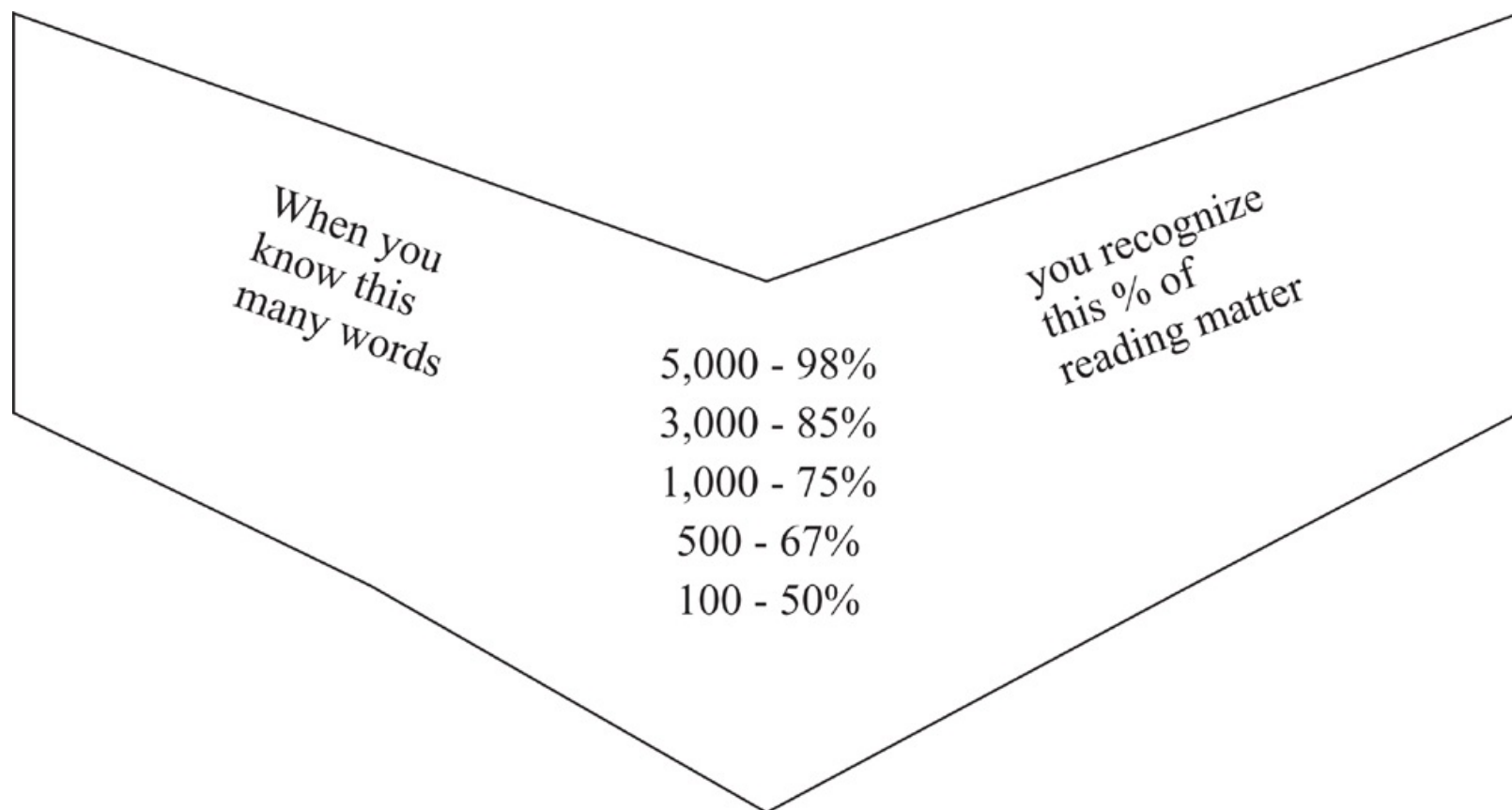
Figure 2. Relationship of Word Frequency to Word Occurrence
